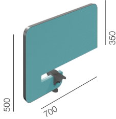
REMOVABLE SIDE SCREEN SS-RM-8550/F W.850 H.500 T.25 mm
