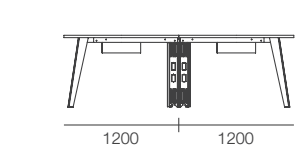
4 SEATER W.2400 D.1500 H.750 mm BLB-D2415/ML1 BLB-D2415/ML2
