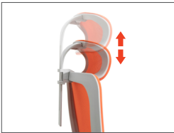
8 Adjustable Headrest (Height Adjustment 90 mm)
