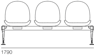
3 Seats W.1790 D.580 H.850 mm Fabric NORDIC-3S/F Scientific Leather NORDIC-3S/VN
