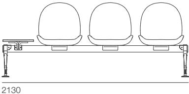
3 Seats with Right Tray W.2130 D.580 H.850 mm Fabric NORDIC-3SPR/F Scientific Leather NORDIC-3SPR/VN
