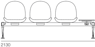
3 Seats with Left Tray W.2130 D.580 H.850 mm Fabric NORDIC-3SPL/F Scientific Leather NORDIC-3SPL/VN
