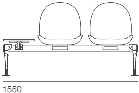
2 Seats with Right Tray W.1550 D.580 H.850 mm Fabric NORDIC-2SPR/F Scientific Leather NORDIC-2SPR/VN
