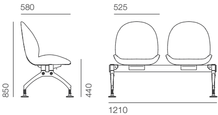
2 Seats W.1210 D.580 H.850 mm Fabric NORDIC-2S/F Scientific Leather NORDIC-2S/VN
