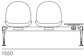
2 Seats with Left Tray W.1550 D.580 H.850 mm Fabric NORDIC-2SPL/F Scientific Leather NORDIC-2SPL/VN
