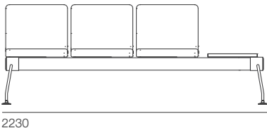
3 Seats with Left Tray NV-09 W.2230 D.600 H.840 mm
