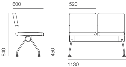
2 Seats NV-06 W.1130 D.600 H.840 mm
