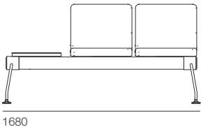
2 Seats with Right Tray NV-14 W.1680 D.600 H.840 mm
