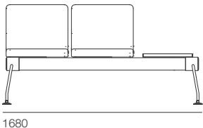
2 Seats with Left Tray NV-13 W.1680 D.600 H.840 mm
