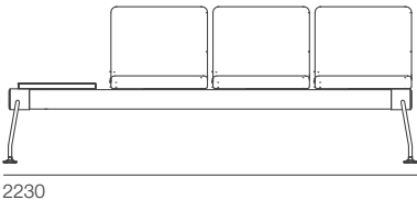
3 Seats with Right Tray NV-10 W.2230 D.600 H.840 mm
