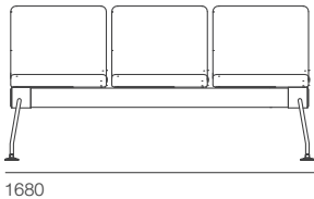
3 Seats NV-07 W.1680 D.600 H.840 mm
