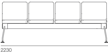
4 Seats NV-08 W.2230 D.600 H.840 mm
