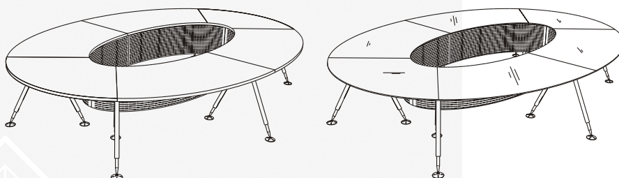
10 SEATS F-CO2638 W 3800 D 2650 H 730 mm
