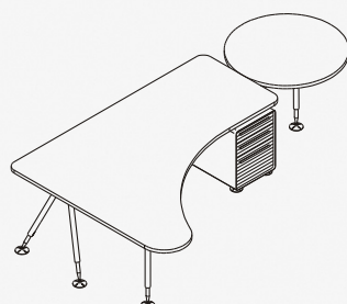
DESK, with Connected Meeting Table and Supporting Drawer F-BO203D (R/L) W 2000 D 1600 H 730 mm F-R90P W 900 H 730 mm
