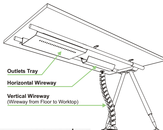
HORIZONTAL WIREWAY (Attach to the Beam Under Worktop) I-HW38 W 380 D 80 H 50 mm
