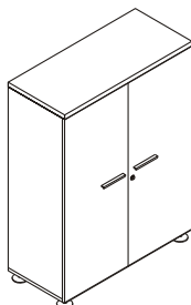
2-DOOR STORAGE CABINET 2 Adjustable Shelves I3-1202 W 900 D 400 H 1250 mm
