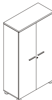
2-DOOR STORAGE CABINET 1 Shelf 2 Adjustable Shelves I3-1602 W 900 D 400 H 1650 mm
