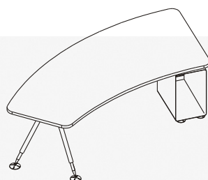
DESK, with Supporting CPU Storage F-C22CP (R/L) W 2240 D 960 H 730 mm
