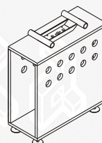
SUPPORTING CPU STORAGE I2-CPU02 W 250 D 770 H 630 mm (Height NOT include connector)
