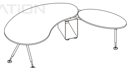
DESK, with Return Worktop and Supporting CPU Storage F-M20CP (R/L) W 2000 D 1050 H 730 mm F-M22CP (R/L) W 2200 D 1050 H 730 mm F-RO120 W 1200 D 600 H 730 mm
