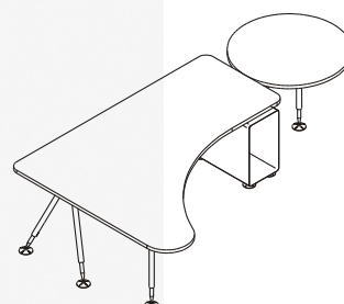
DESK, with Connected Meeting Table and Supporting CPU Storage F-BO20CP (R/L) W 2000 D 1600 H 730 mm F-R90P W 900 H 730 mm
