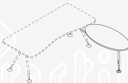
RETURN WORKTOP F-RO120 W 1200 D 600 H 730 mm
