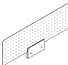
DESK'S TOP SCREEN, Perforated Steel FMD-MS4012 W 1200 H 400 T 2 mm
