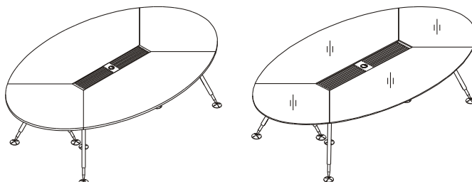
8 SEATS F-CO1628 W 2800 D 1600 H 730 mm
