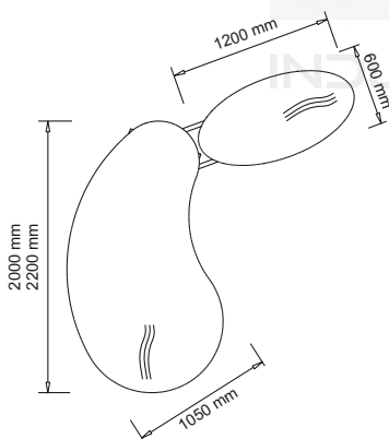
DESK, with Return Worktop and Supporting Drawer F-M203D (R/L) W 2000 D 1050 H 730 mm F-M223D (R/L) W 2200 D 1050 H 730 mm F-RO120 W 1200 D 600 H 730 mm
