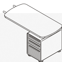
RETURN WORKTOP with Supporting Drawer F-RE123D (R/L) W 1200 D 600 H 730 mm
