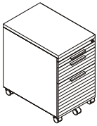
MOBILE DRAWER 1 Pencil Drawer 1 Small Drawer 1 Hanging File Drawer I2-653FR W 420 D 570 H 630 mm
