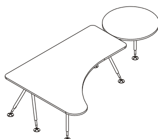
DESK, with Connected Meeting Table F-BO2000 (R/L) W 2000 D 1600 H 730 mm F-R90P W 900 H 730 mm
