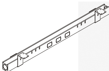
HORIZONTAL WIREWAY (Attach Under Worktop) I-HW100 W 1000 D 80 H 100 mm I-HW120 W 1200 D 80 H 100 mm I-HW160 W 1600 D 80 H 100 mm
