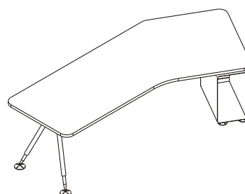
DESK, with Supporting CPU Storage F-J22CP (R/L) W 2200 D 960 H 730 mm F-J24CP (R/L) W 2400 D 960 H 730 mm
