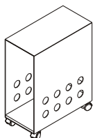
MOBILE CPU STORAGE I-CPU01R W 250 D 500 H 630 mm
