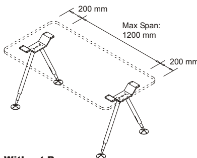
Without Beam Maximum span = 1200 mm Maximum worktop length = 1600 mm
