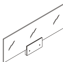
DESK'S TOP SCREEN, Laminated Glass FMD-GS4012 W 1200 H 400 T 6 mm
