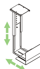
SUSPENDED CPU STORAGE (Adjustable Height and Width) I-CPU04 W 205-305 D 240 H 320-535 mm
