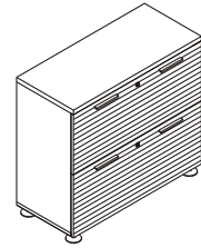
HANGING FILE STORAGE 2 Hanging File Drawer (2 x 2 Rows) I2-800F W 900 D 400 H 850 mm
