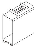
SUPPORTING CPU STORAGE F-CPU02 W 250 D 770 H 630 mm (Height NOT include connector)
