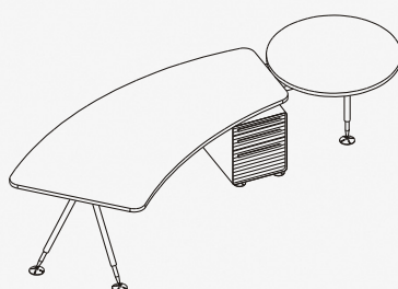
DESK, with Connected Meeting Table and Supporting Drawer F-CS223D (R/L) W 2240 D 960 H 730 mm F-R90P W 900 H 730 mm
