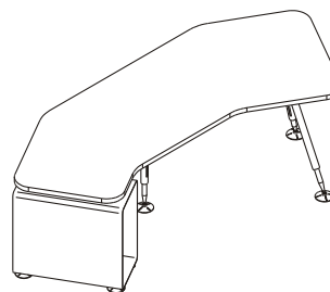
DESK, with Supporting CPU Storage F-U22CP (R/L) W 2200 D 800 H 730 mm F-U24CP (R/L) W 2400 D 800 H 730 mm
