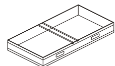
HANGING FILE FRAME (To Install Inside 2-Door Storage Cabinet) I-HF9040 W 860 D 355 H 100 mm
