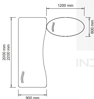
DESK, with Return Worktop F-CR2000 W 2000 D 900 H 730 mm F-CR2200 W 2200 D 900 H 730 mm F-RO120 W 1200 D 600 H 730 mm
