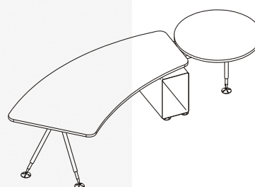
DESK, with Connected Meeting Table and Supporting CPU Storage F-CS22CP (R/L) W 2240 D 960 H 730 mm F-R90P W 900 H 730 mm
