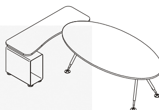
DESK, with Return Worktop and Supporting CPU Storage F-O2000 W 2000 D 1100 H 730 mm F-RES16CP (R/L) W 1600 D 600 H 730 mm
