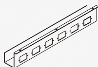
HORIZONTAL WIREWAY (Attach Under Worktop) HW80 W 800 D 80 H 90 mm HW100 W 1000 D 80 H 90 mm HW120 W 1200 D 80 H 90 mm HW160 W 1600 D 80 H 90 mm
