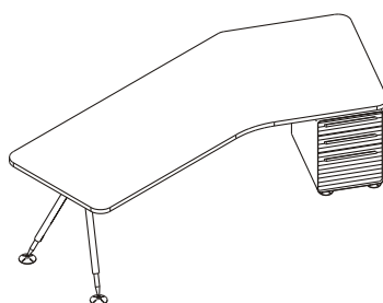
DESK, with Supporting Drawer F-J223D (R/L) W 2200 D 960 H 730 mm F-J243D (R/L) W 2400 D 960 H 730 mm
