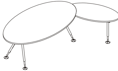
DESK, with Return Worktop F-O2200 W 2200 D 1100 H 730 mm F-ROS110 (R/L) W 1100 D 600 H 730 mm
