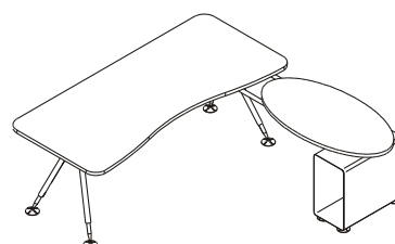
DESK, with Return Worktop and Supporting CPU Storage F-CR2000 W 2000 D 900 H 730 mm F-CR2200 W 2200 D 900 H 730 mm F-RO12CP (R/L) W 1200 D 600 H 730 mm
