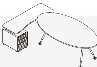
DESK, with Return Worktop and Supporting Drawer F-O2000 W 2000 D 1100 H 730 mm F-RES163D (R/L) W 1600 D 600 H 730 mm
