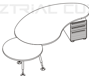
DESK, with Connected Meeting Table and Supporting Drawer F-M203D (R/L) W 2000 D 1050 H 730 mm F-M223D (R/L) W 2200 D 1050 H 730 mm F-RS90P W 900 H 730 mm
