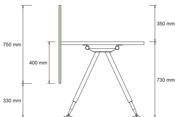
Standard Height Screen: 750 mm
