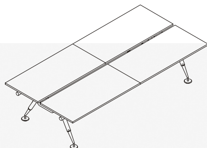
4 SEATS F-MD3200-A W 3200 D 1600 H 730 mm
