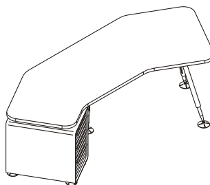
DESK, with Supporting Drawer F-U223D (R/L) W 2200 D 800 H 730 mm F-U243D (R/L) W 2400 D 800 H 730 mm
