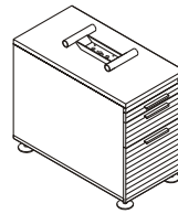
SUPPORTING DRAWER 1 Pencil Drawer 1 Small Drawer 1 Hanging File Drawer I2-673F W 420 D 770 H 630 mm (Height NOT include connector)
